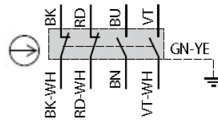
ZCWD41L... / XCWD41...L...
