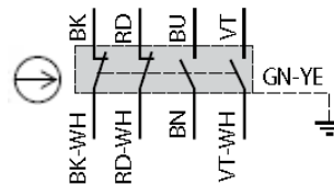
ZCWD41L... / XCWD41...L...
