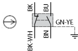
ZCWD21L... / XCWD21...L...
